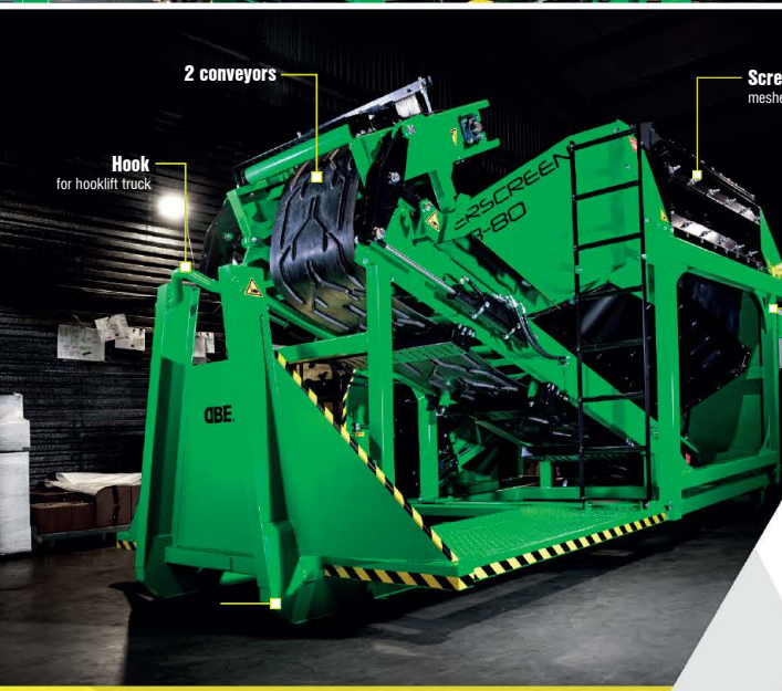
Frame high-strength steel construction ensures maximum stability
